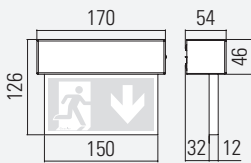
DR1Ö EYELET MOUNTING
