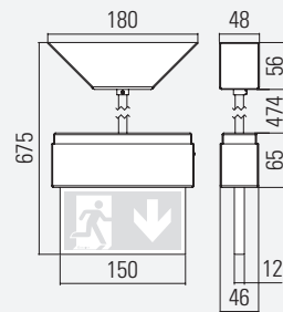
DR1P PENDANT MOUNTING
