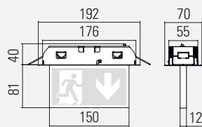
DR1E RECESSED CEILING MOUNTING JUNCTION BOX FOR DR1E
