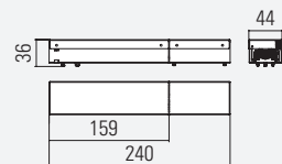
DR1E RECESSED CEILING MOUNTING JUNCTION BOX FOR DR1E
