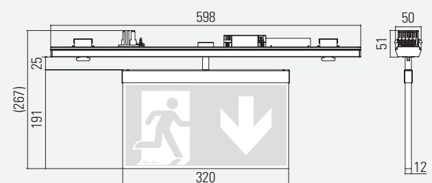
EXIT SIGN LUMINAIRE (31 m)
